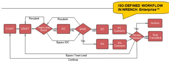
Fig 3. Example of workflow creation (using WRENCH Enterprise™ workflow drawing feature).
